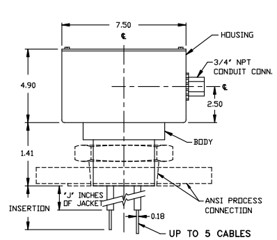
Model P43 Multiple Cable Probe, Integral Electronics Unit
