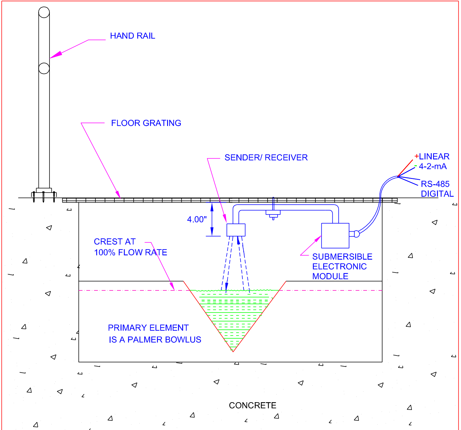
OPEN CHANNEL FLOW MEASUREMENT IN A SHALLOW, UNDER- THE-FLOOR, CHANNEL WITH VERY LITTLE HEAD ROOM; M/N 871FM-- CITY OF SAN JOSE, CA.
