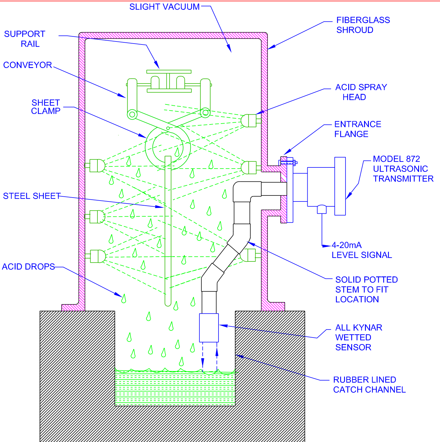
CONTROLLING ACID LEVEL IN A STEEL SHEET PICKLING LINE WITH A MODEL 872 ULTRASONIC- LUKENS STEEL
