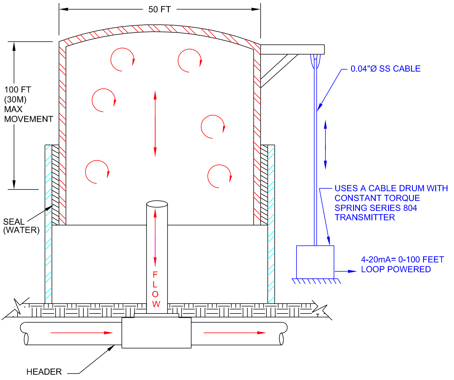
MEASURING THE VOLUME (HEIGHT) OF A LARGE BLAST FURNACE GAS HOLDER U.S. STEEL- SPARROW POINT MILL
