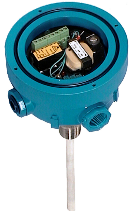
Model 105 in Hoseproof Housing with cover removed
